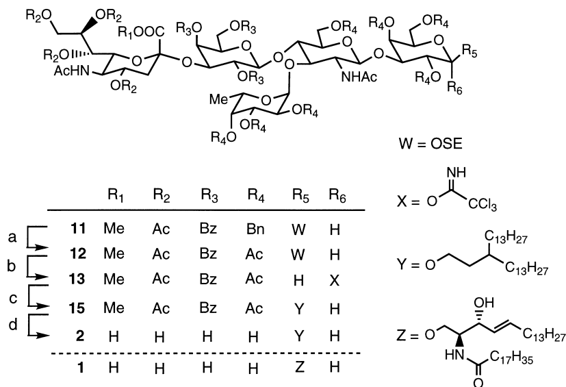
Scheme 2. Reagents: (a) \text{H}_2/10\%\text{Pd/C} , \text{Ac}_2\text{O/pyridine} , DMAP (75%); (b) (i) \text{CF}_3\text{CO}_2\text{H} , \text{CHCl}_3 (93%), (ii) \text{CCl}_3\text{CN/DBU} , \text{CHCl}_3 (85%); (c) 3-tridecylhexadecanol ( 14 ), \text{BF}_3/\text{OEt}_2 , \text{CH}_2\text{Cl}_2 (74%); (d) \text{NaOMe} , \text{MeOH} (100%).
